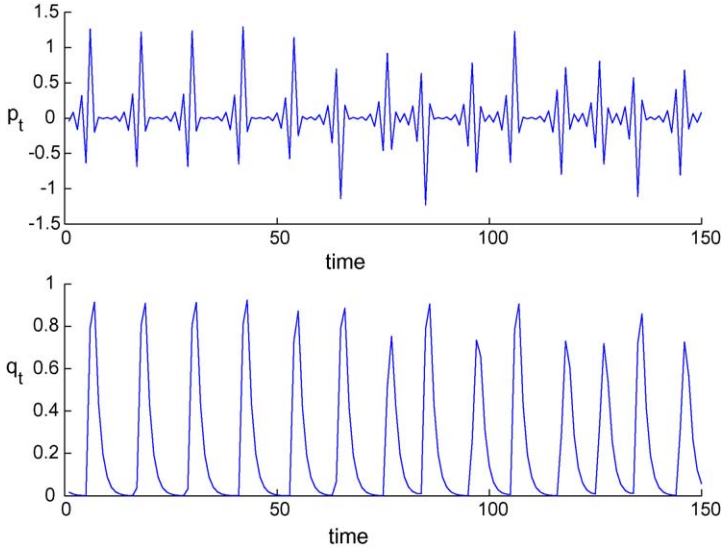
Fig. 6. Trajectory for (p_t, q_t) when b/B=2 and \alpha=2.3 .
