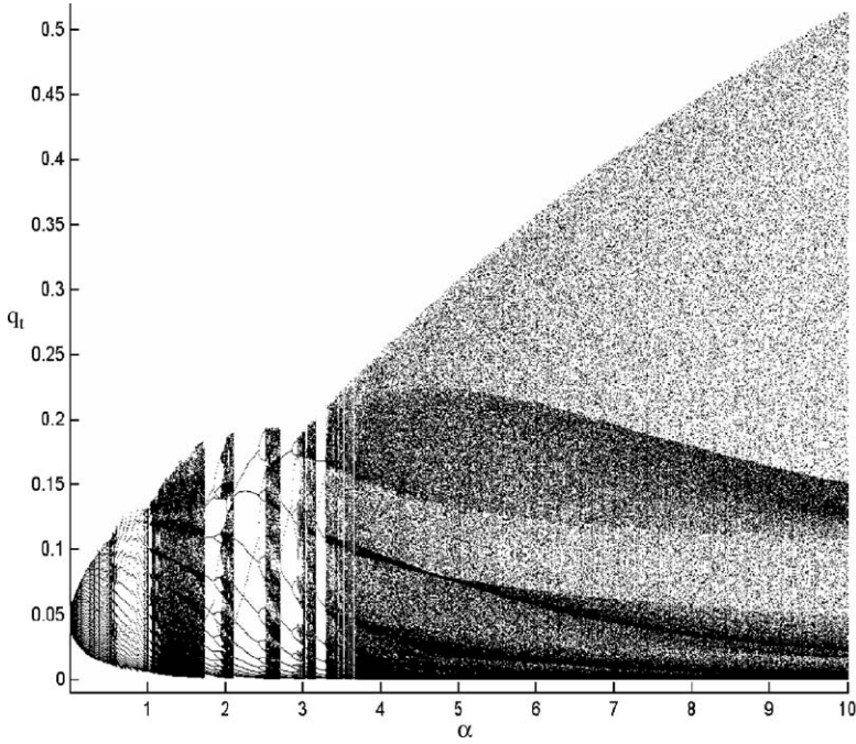
Fig. 1. Bifurcation diagram for q_t when b/B=1.1 .
