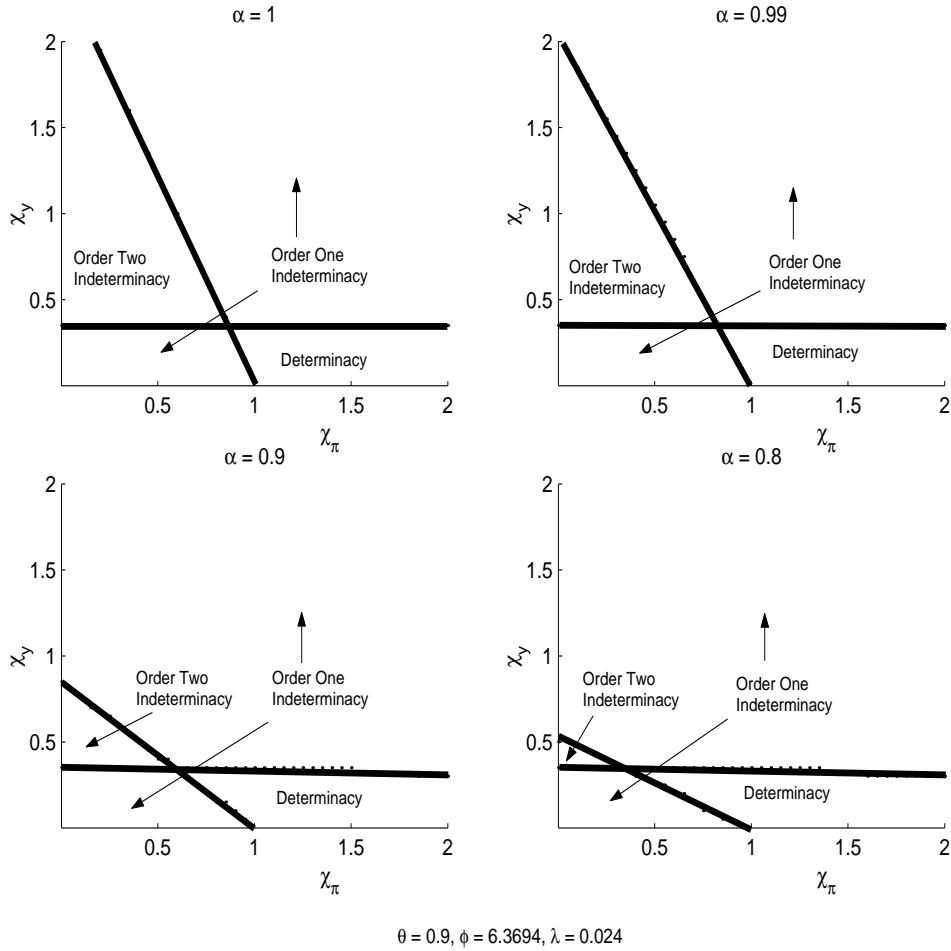
Figure 1: Determinacy Properties: \theta \leq 1 .
