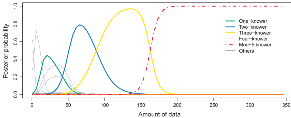
Fig. 6. Learning results for a Mod-5 system.
