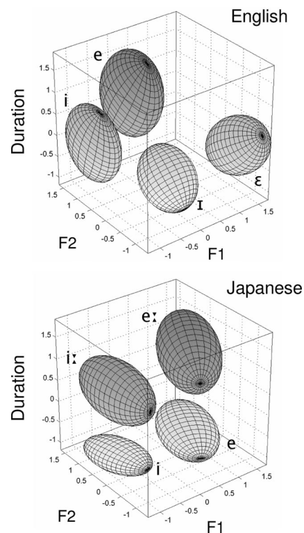
Fig. 1. The Gaussian distributions for the English /i/, /e/, /ɪ/, /ɛ/ and Japanese /i:/, /e:/, /e/, computed over the read vowels from all speakers (the tokens were z-scored for each speaker before the analysis). The ellipsoids are equal-probability surfaces, 1 SD along each principal axis, enclosing \approx 19\% of the total probability mass. Note that these are aggregate tendencies; the vowel categories of individual speakers varied greatly, covered a wider range, and overlapped with each other considerably.
