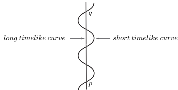
Figure 1. A long timelike curve from p to q and a very short one that swings back-and-forth, and approximates a broken null curve.
