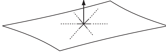
Figure 2. A “geodesic hypersurface” through a point is constructed by projecting geodesics in all directions orthogonal to a given timelike vector there.
