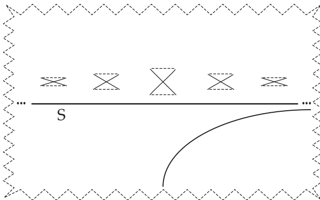
Figure 3: A two-dimensional version of (the covering space of) anti de-Sitter spacetime. The indicated set of world points S seems a plausible candidate for representing “space at a given time”. But it fails to qualify as a spatial class because there are smooth timelike curves without endpoint that “rush off to spatial infinity” before intersecting it.
