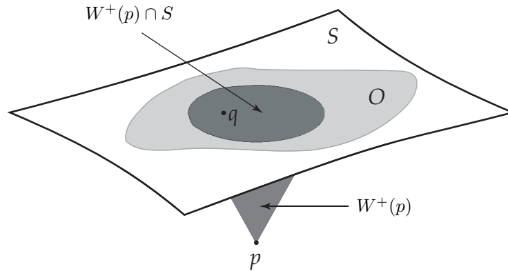
Figure 1: In definition 2, the “open” subsets of a spatial class are defined in terms of W .
