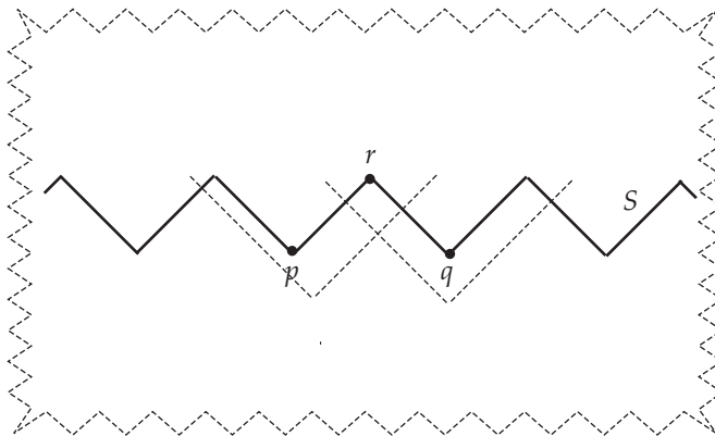
Figure 2: Even if we understand W to be the relation \ll , the W -topology need not be Hausdorff. Here given any “open” subsets of S containing p and q respectively, their intersection contains r .
