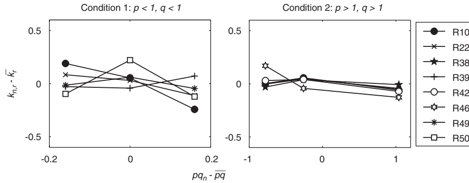
Fig. 1. Experiment 1b: results for testing the k -multiplicative property.
