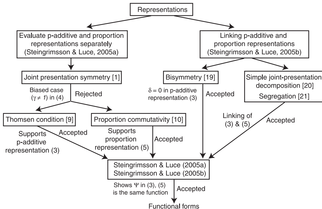
Fig. 2. The diagram summarizes the work reported in Steingrímsson and Luce (2005a, 2005b), the first two articles on the Empirical Evaluation of a Model of Global Psychophysical. Together they provided support for the p -additive (3) and proportion (5) representations that emerged from Luce (2002, 2004).
