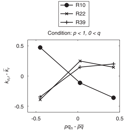
Fig. E1. Experiment 1b: results for testing the k -multiplicative property in the mixed condition p < 1, 0 < q .
