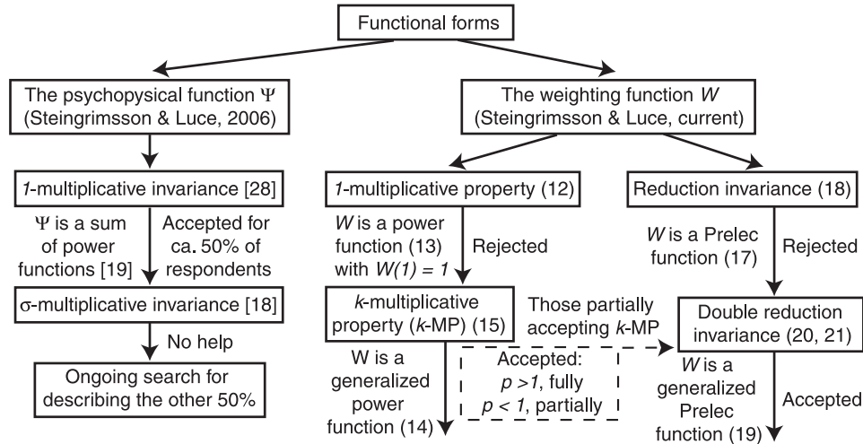
Fig. 3. The diagram summarizes the work reported in Steingrímsson and Luce (2006) and the current article, the third and fourth articles on the Empirical Evaluation of a Model of Global Psychophysical . These two explore possible functional forms for the psychophysical function \Psi and the weighting function W .
