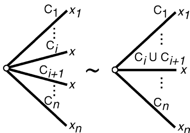
FIGURE 2. A graphical example of coalescing.
