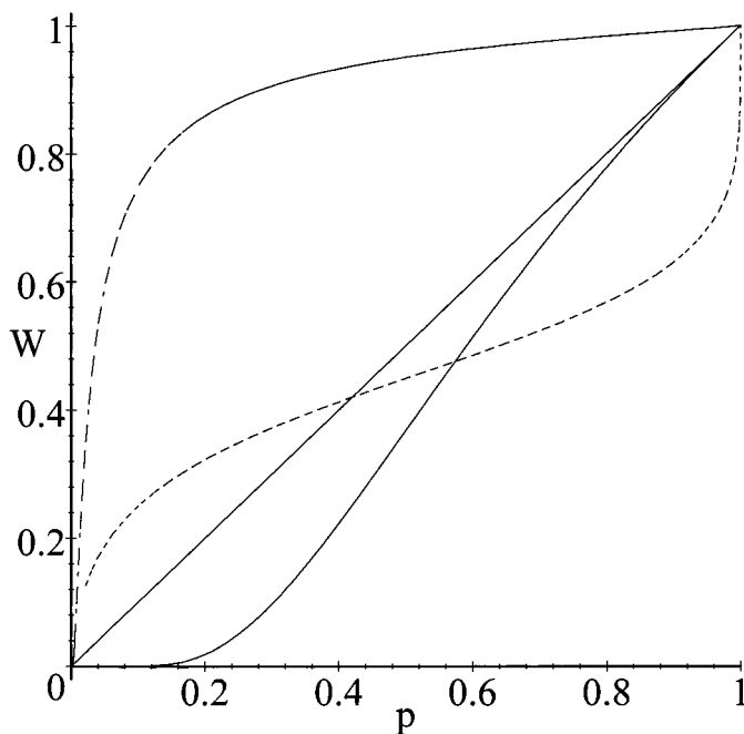
FIG. 1. Plots of W(p) = \exp[-\beta(\frac{1-p}{p})^\alpha] for \alpha = 1, \beta = 1 (solid), \alpha = .25, \beta = .80 (dotted), and \alpha = .80, \beta = .05 (dashed).
