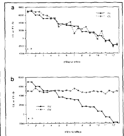
Fig. 4. Plots of certainty equivalents (CEs) and expected values (EVs) across items. The two markers for each item number on the x-axis are gambles a and b, respectively. For most subjects, CE followed EVs closely, as in the data for Subject 20 (a). A few subjects, however, had flat CE curves, as in the data for Subject 3 (b).
