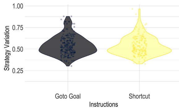
Fig 8. Strategy variation between trials for all subjects. The violin plots show the distribution of strategic variation (SV in Eq. 4). Two hundred and six subjects were instructed to go to the goal location; 162 subjects were instructed to take the shortest path to the goal location.
