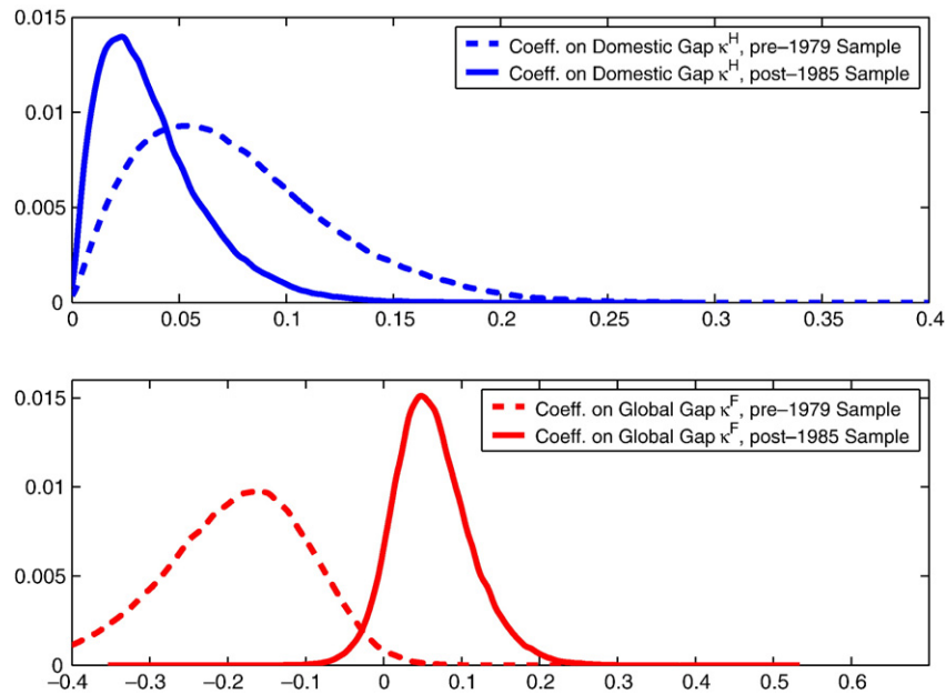
Fig. 2. Posterior distributions across sub-samples: NK Phillips curve coefficients on domestic and 'global' slack.
