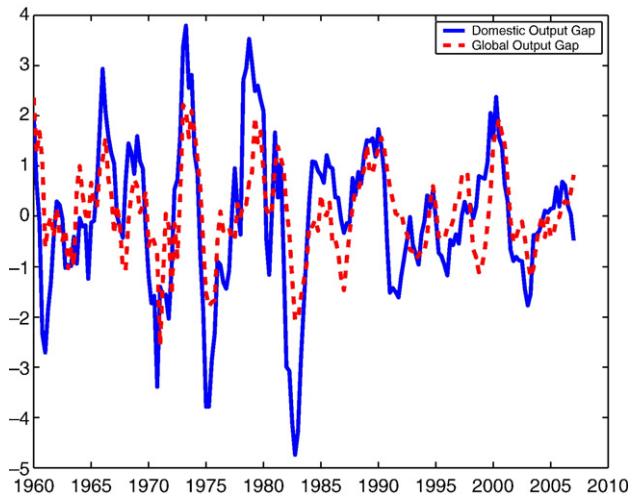
Fig. 1. Domestic and 'global' output gap series.
